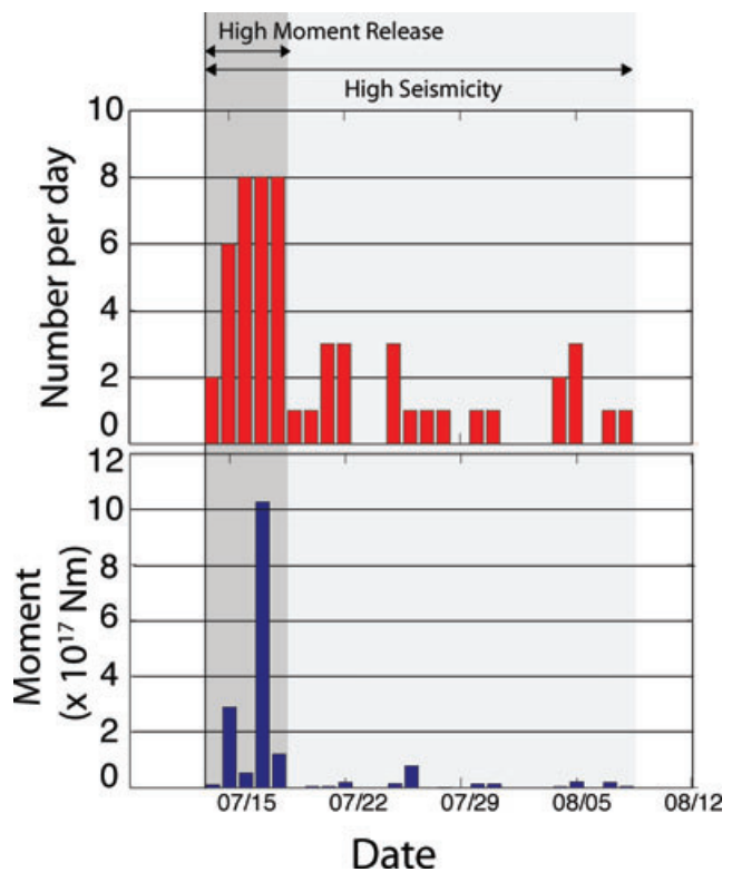
Figure 3. Seismicity during the 2007 Lake Natron Seismic Swarm. Daily earthquake numbers and moment through time as recorded by the NEIC PDE catalogue. The swarm lasted for 22 d, but the majority of the moment was released during the first 5 d.
