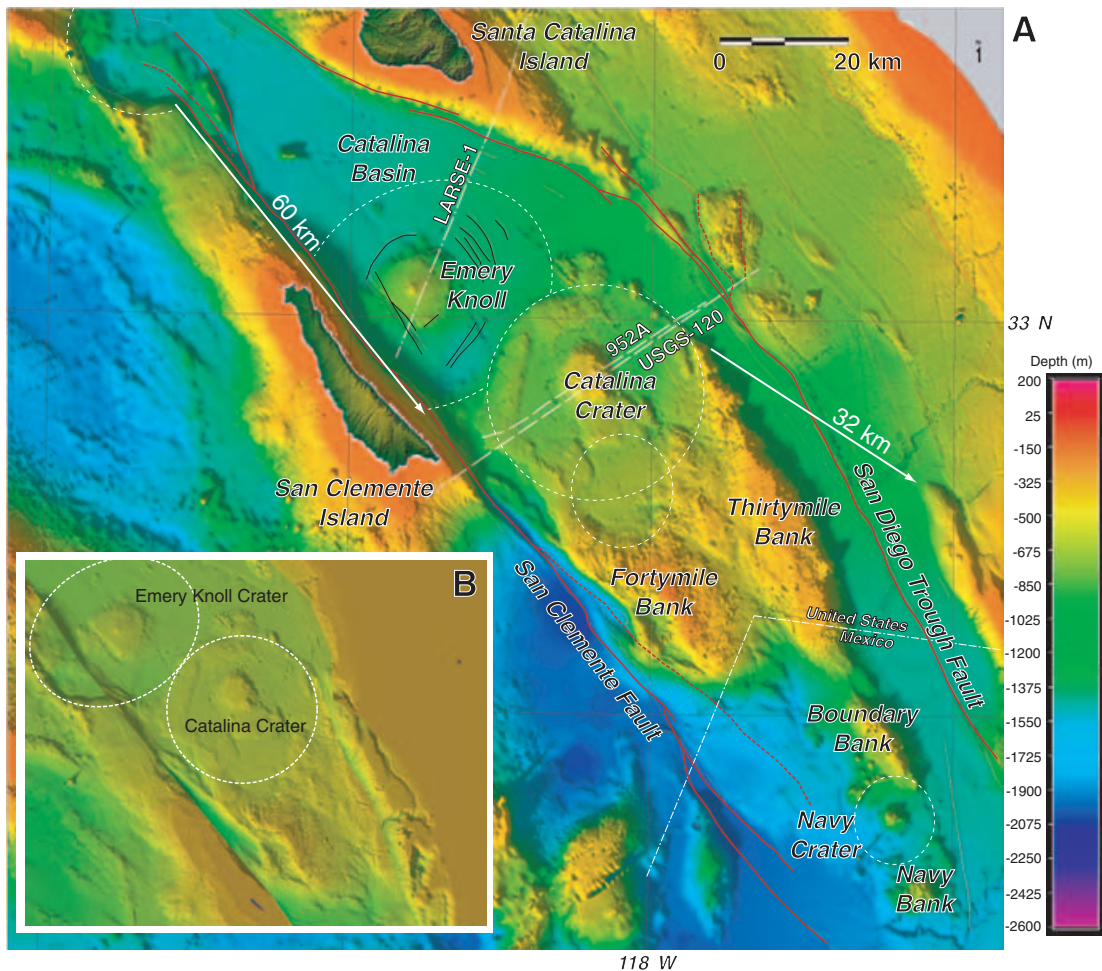
Figure 2. (a) Shaded relief bathymetry of Inner California Borderland showing location of inferred crater structures (white), active faults (red), older faults (black) and white displacement vectors used to create palinspastic map shown in (b) (Legg et al. 2002). Dashed circles outline inferred crater outer rims and a possible secondary feature that overlaps Catalina Crater to the south. Note ring fault segments around Emery Knoll mapped by Junger & Vedder (1980) and Vedder et al. (1986). (b) Palinspastic reconstruction after 60 km of right slip along San Clemente fault and 32 km of right oblique extension across San Diego Trough have been removed. After reconstruction, the inferred western outer rim of Emery Knoll Crater is restored.
